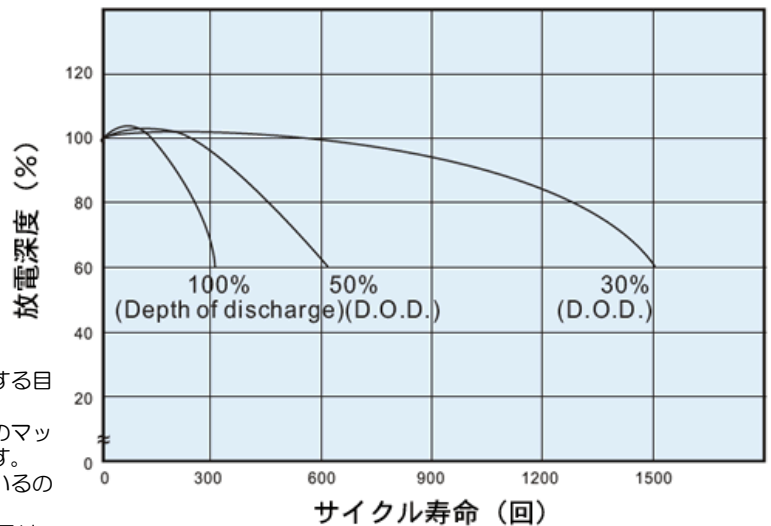
Battery Life Characteristics of Cyclic Use
